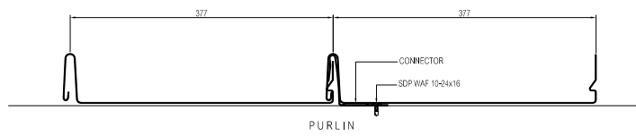
SECTION DETAIL 1" SCALE 1:8
